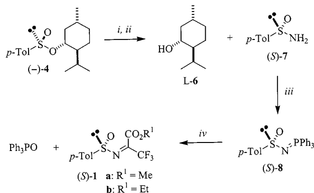
Scheme 4. Key: i) LiHMDS, THF, -70^\circ\text{C} ; ii) \text{NH}_4\text{Cl}/\text{H}_2\text{O} ; iii) \text{PPh}_3 , DEAD, THF, room temp. (92%); iv) \text{CF}_3\text{COCO}_2\text{R}^1 , PhH distilled from Na, 40^\circ\text{C}
