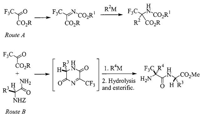
Scheme 1. Routes to \alpha -Tfm \alpha -amino acids
