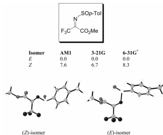
Figure 1. Theoretical calculations on sulfinimine ( S )- 1a (energies are in kcal/mol)
