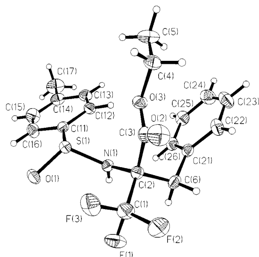
Figure 5. ORTEP diagram of (±)-13b
