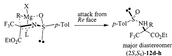
Figure 3. Chelation control (Wills' model)
