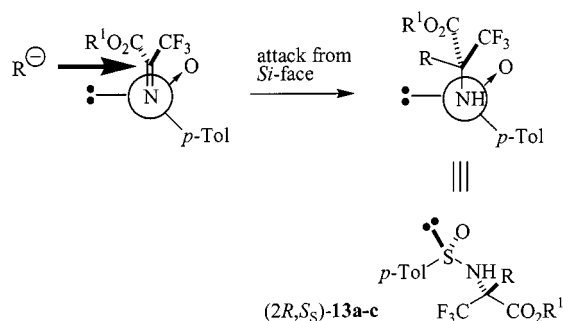
Figure 4. Non-chelation control (Fujisawa's model)
