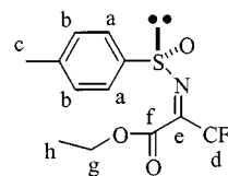
Figure 2. The more stable ( E ) isomer of sulfinimine ( S )- 1b
