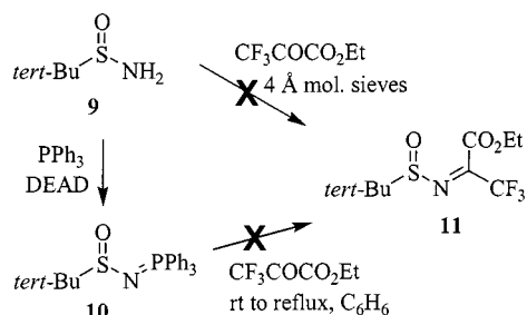
Scheme 5. Attempts to obtain tert -butylsulfinylimine 11
